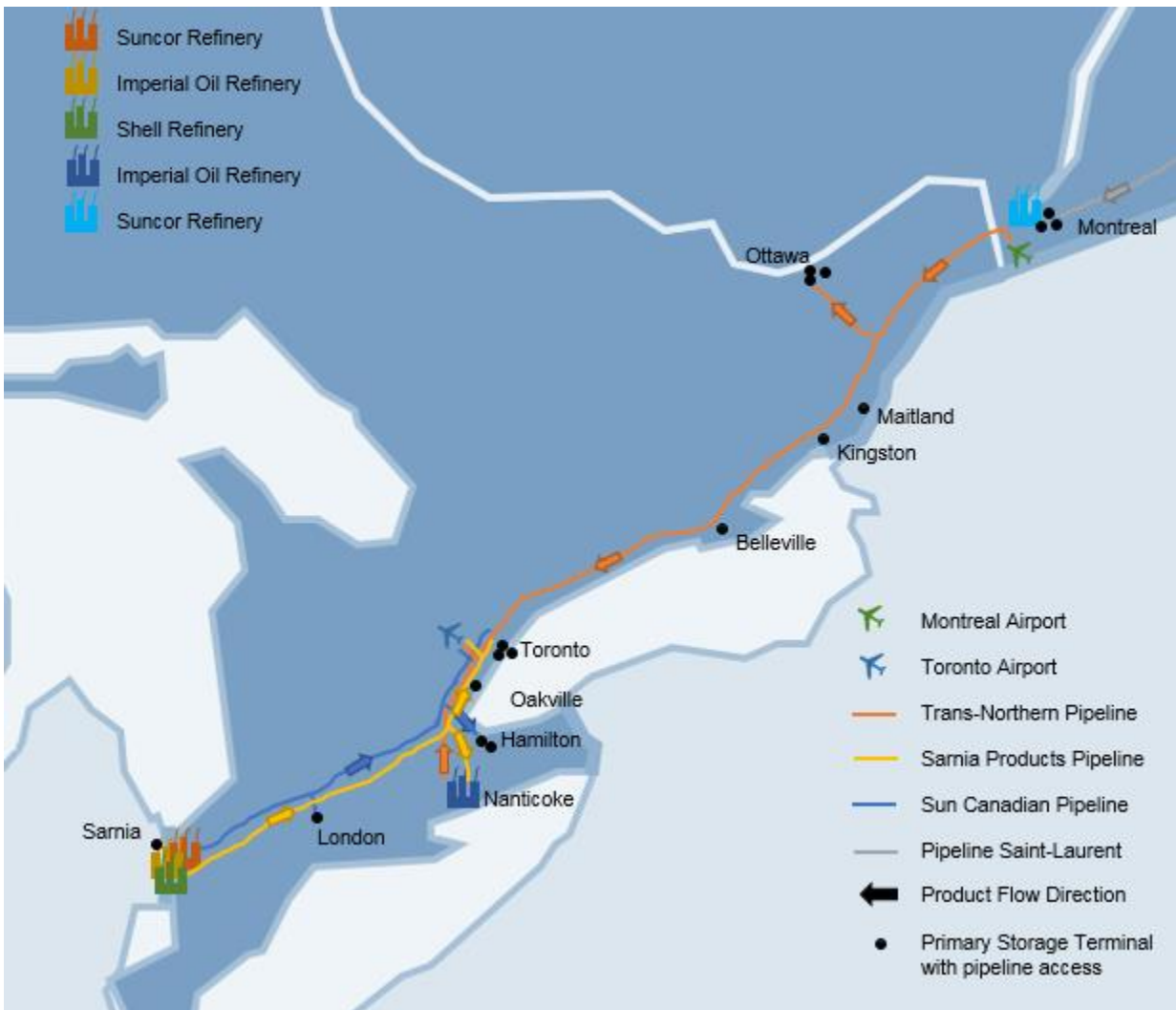
Figure 8: Refined product pipelines in Central Canada
