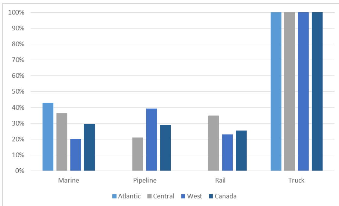
Figure 12: Percentage of Primary Terminals with each type of Product Discharge Capability by Region.
