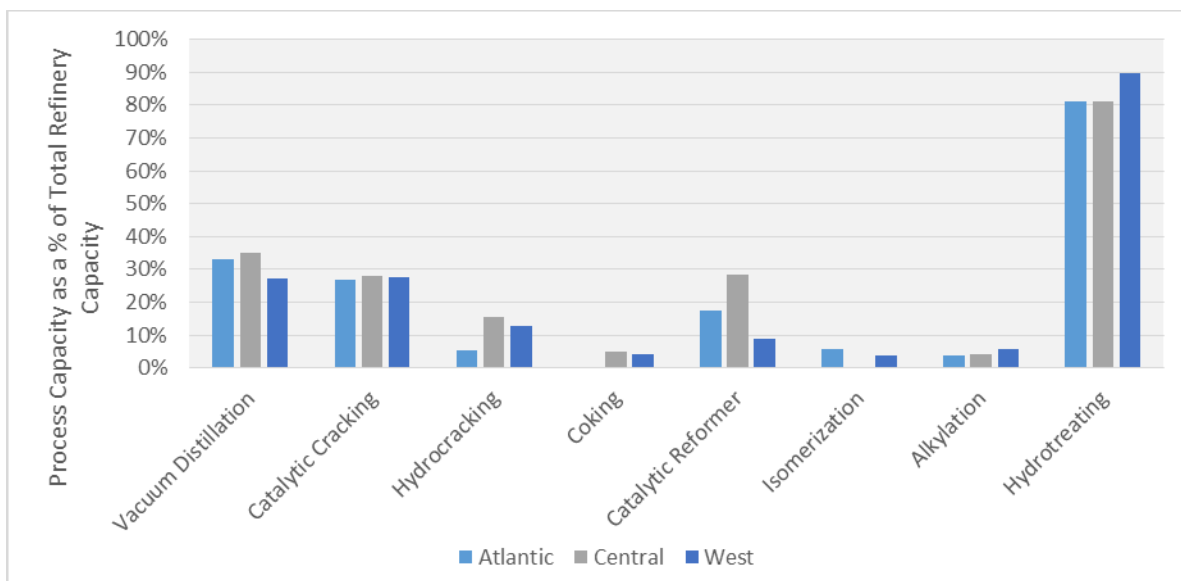
Figure 5: Process Unit Capacity as a Percentage of Total Refinery Capacity - by region
